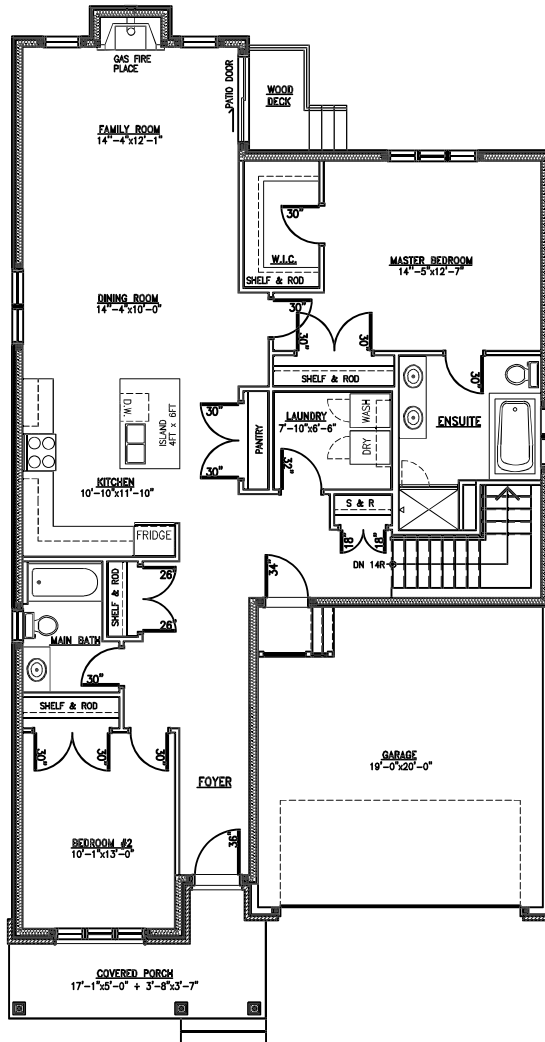
MainFloor
