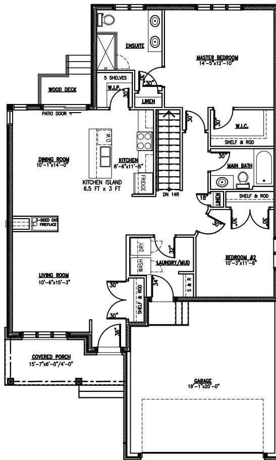
Main Floor
