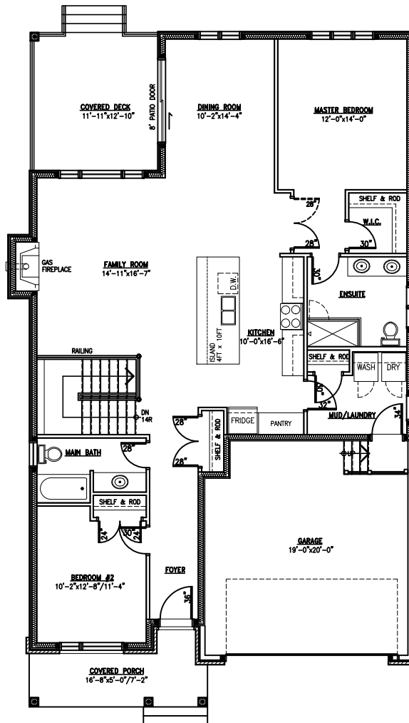
MainFloor
