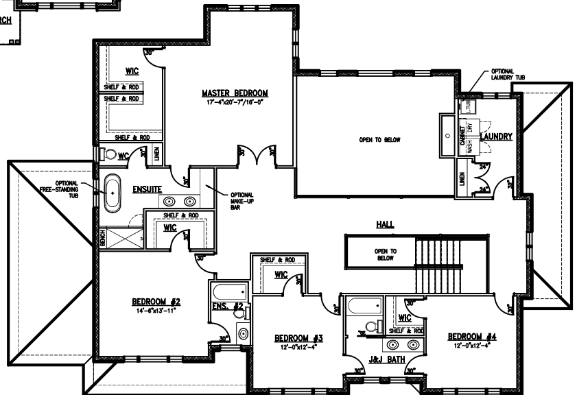
Second Floor
