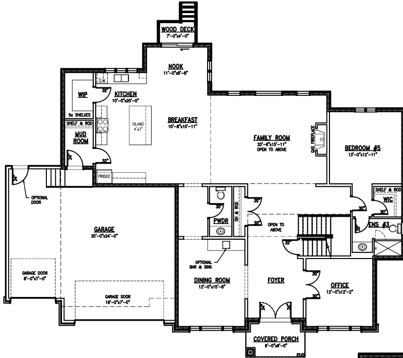
Main Floor
