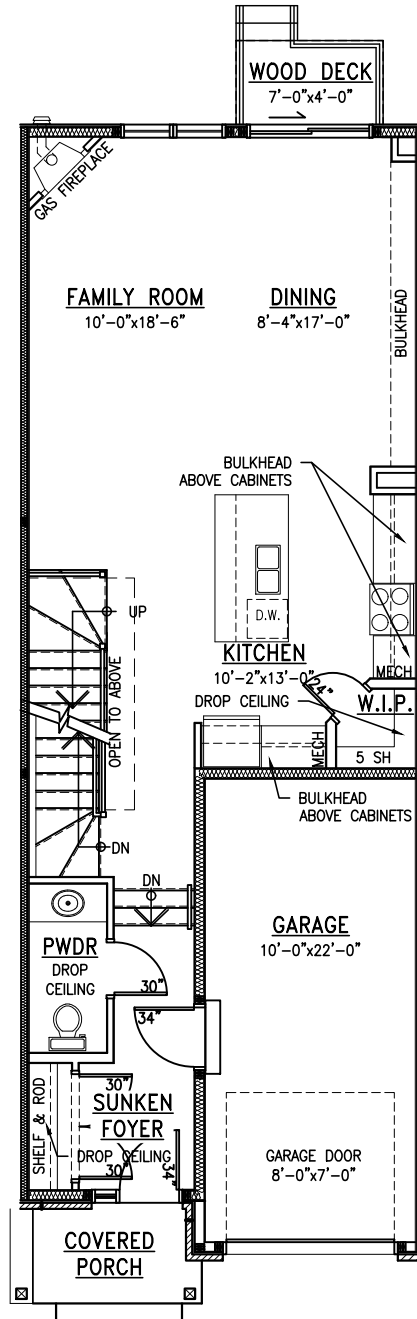
Main Floor
