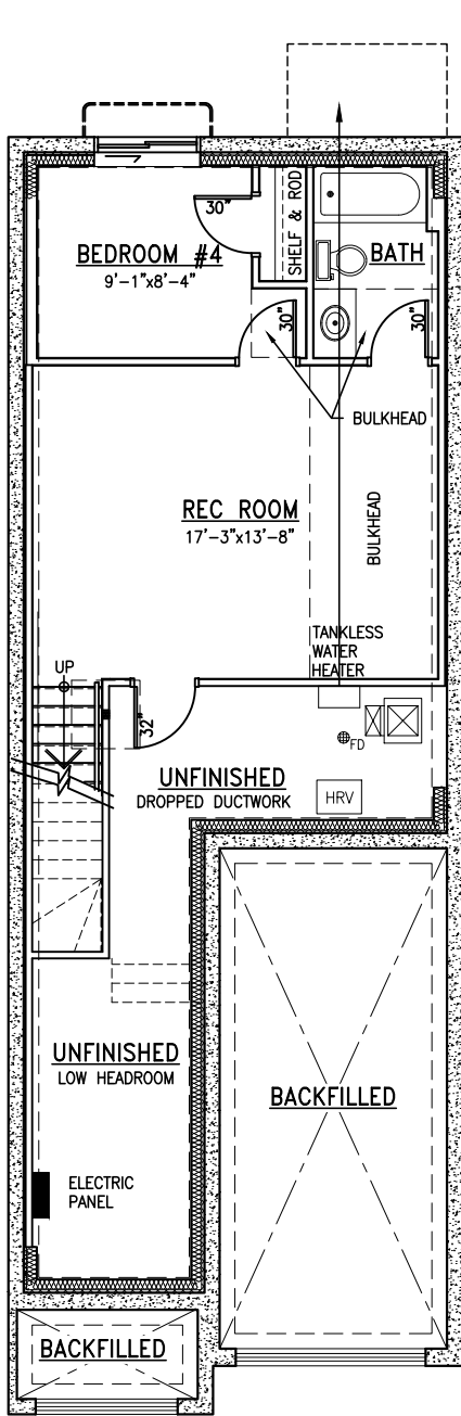
Basement
