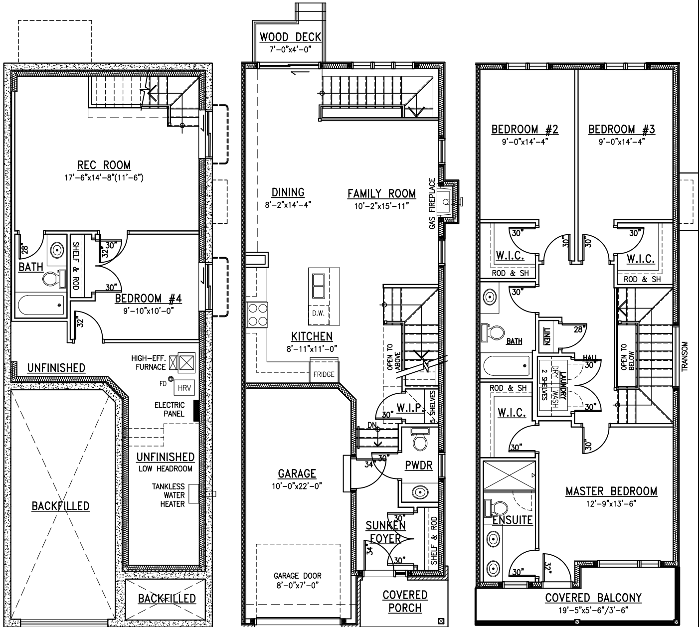
Basement
