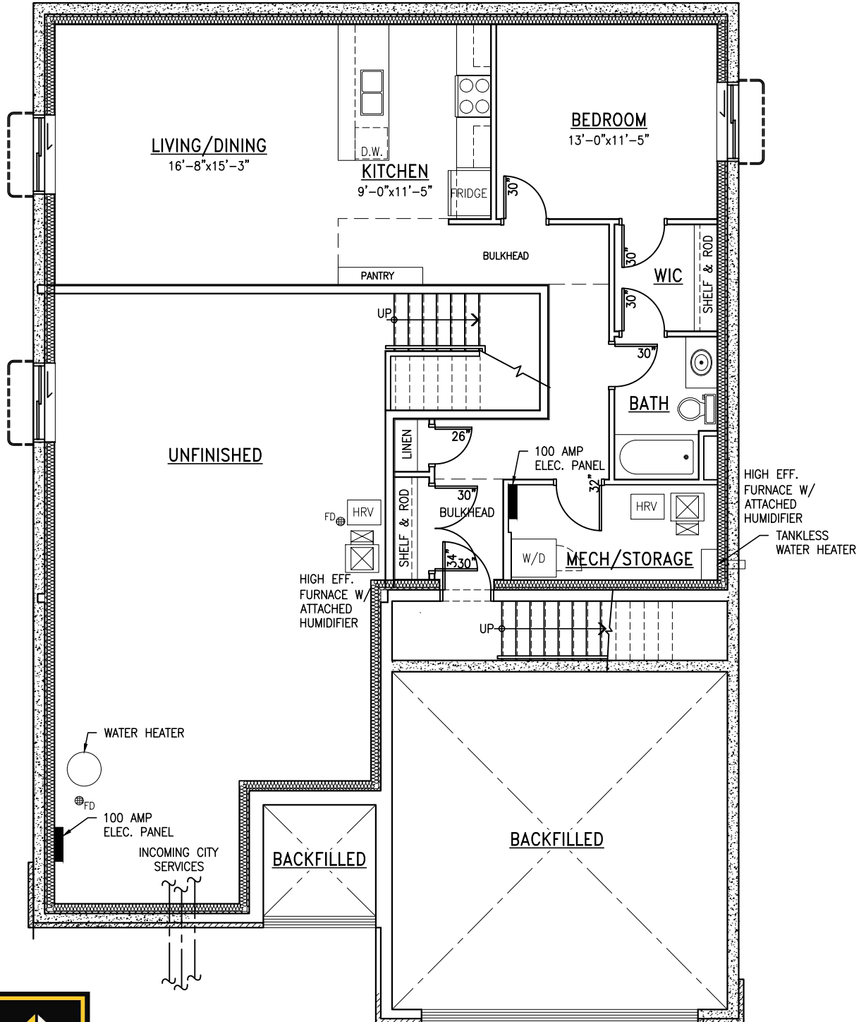
Basement Additional Dwelling Unit - 810 SQFT
