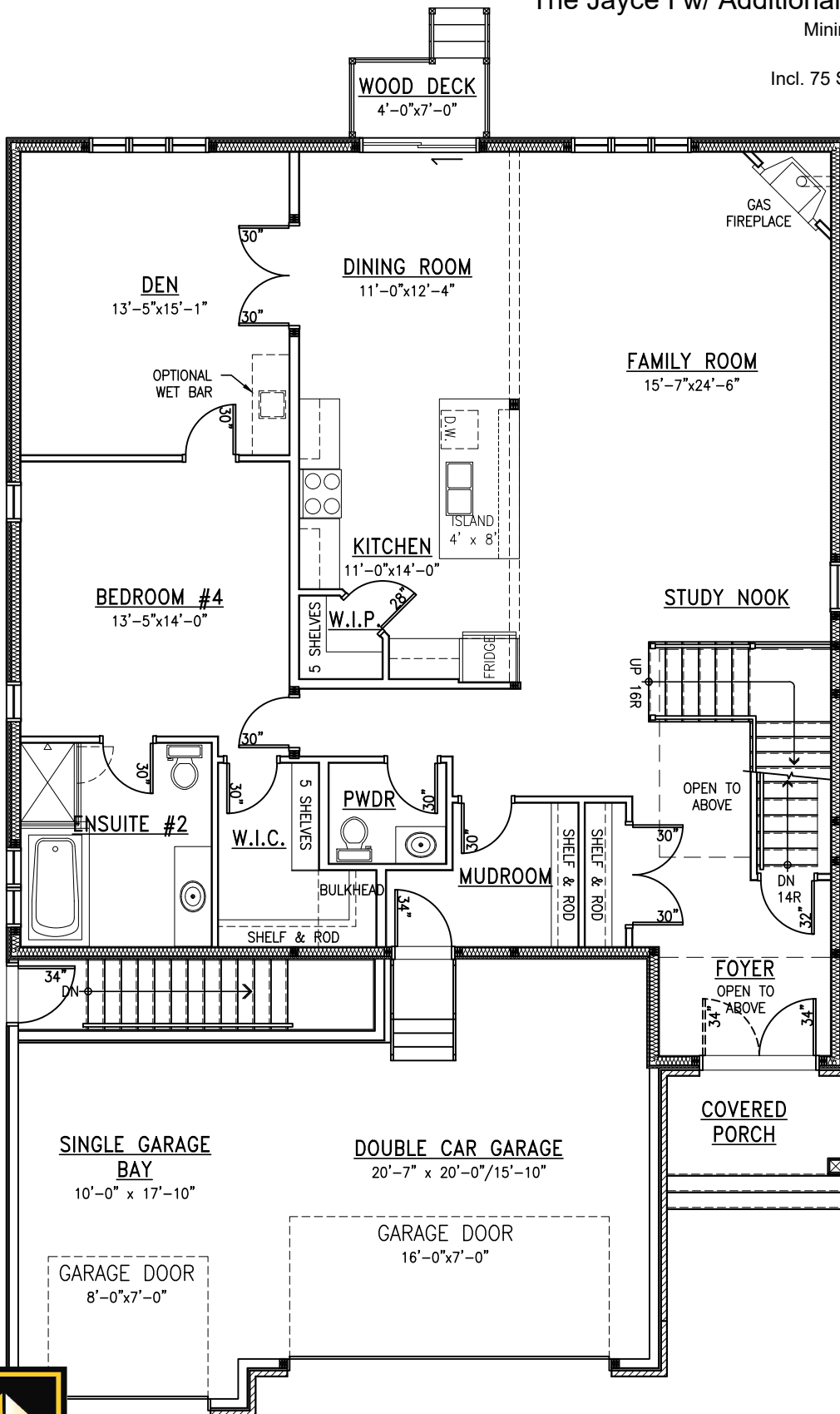
Main Floor
