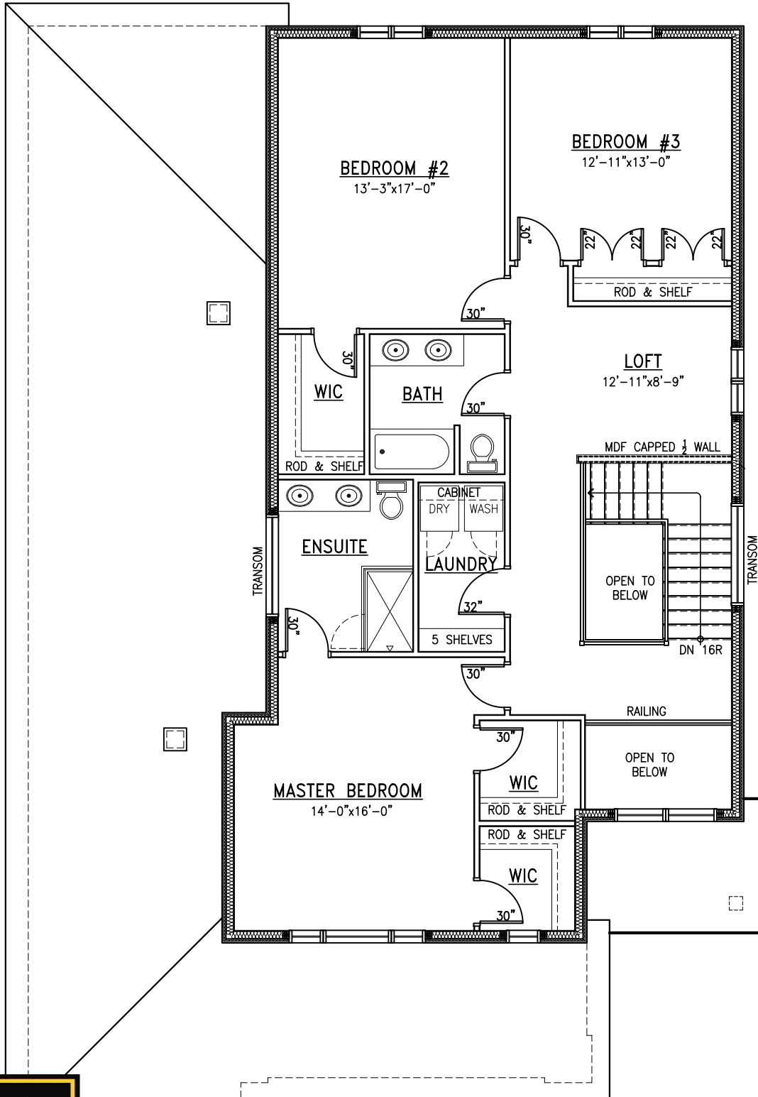
Second Floor
